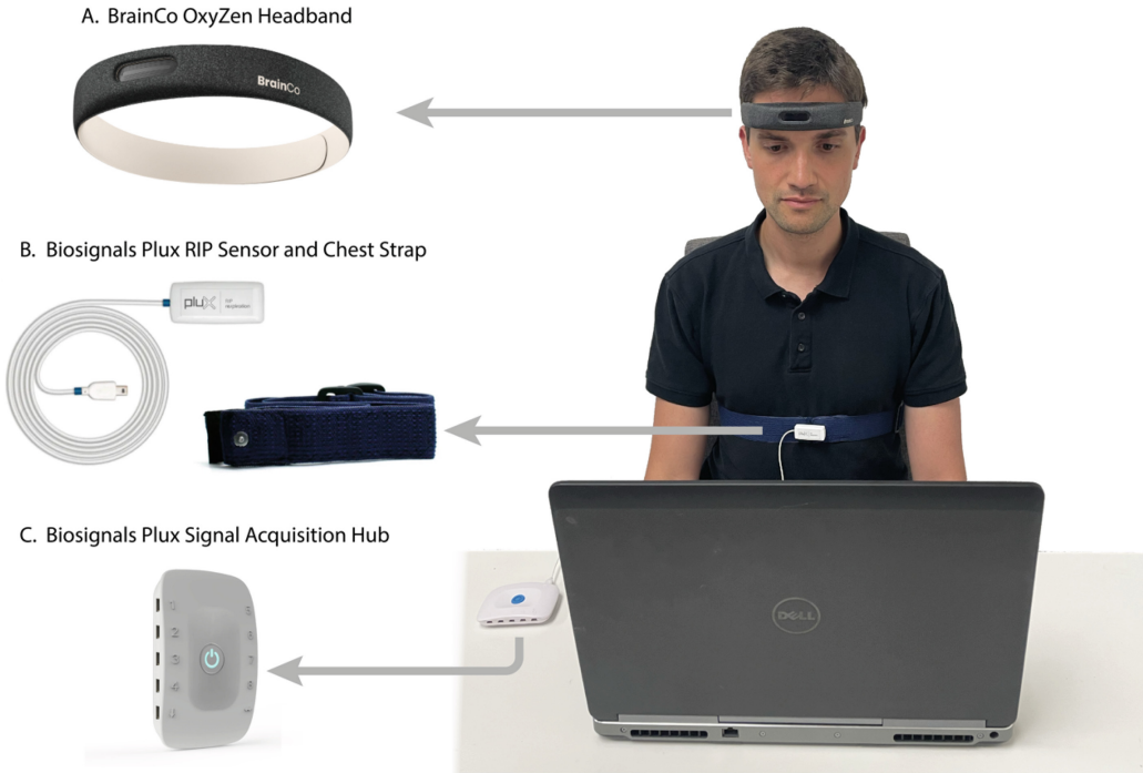
Fig. 2. Experimental setup: Subjects were instructed to breathe normally while synchronized data of A) PPG sensor embedded in BrainCo’s OxyZen headband and B) Biosignals Plux RIP sensor in conjunction with C) a signal acquisition hub were collected.
