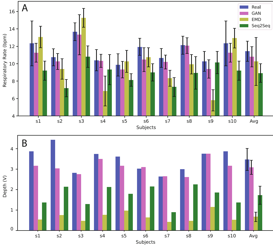
Fig. 9. Breathing measures: A) Average RR estimation over 1 min test signal, based on the generated signals by three models are compared with RR of ground-truth for all subjects individually as well as average over all subjects. B) Depth scores for generated signals and the ground-truth curve are compared for all individual subjects and average of all subjects. These graphs shows the superior performance of GAN-generated signal in monitoring breathing pattern.
